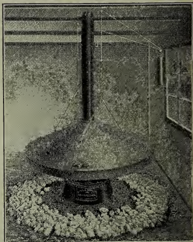
IDEAL BROODER STOVE.
